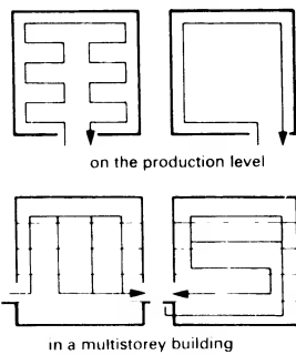
⑥ Materials flow
